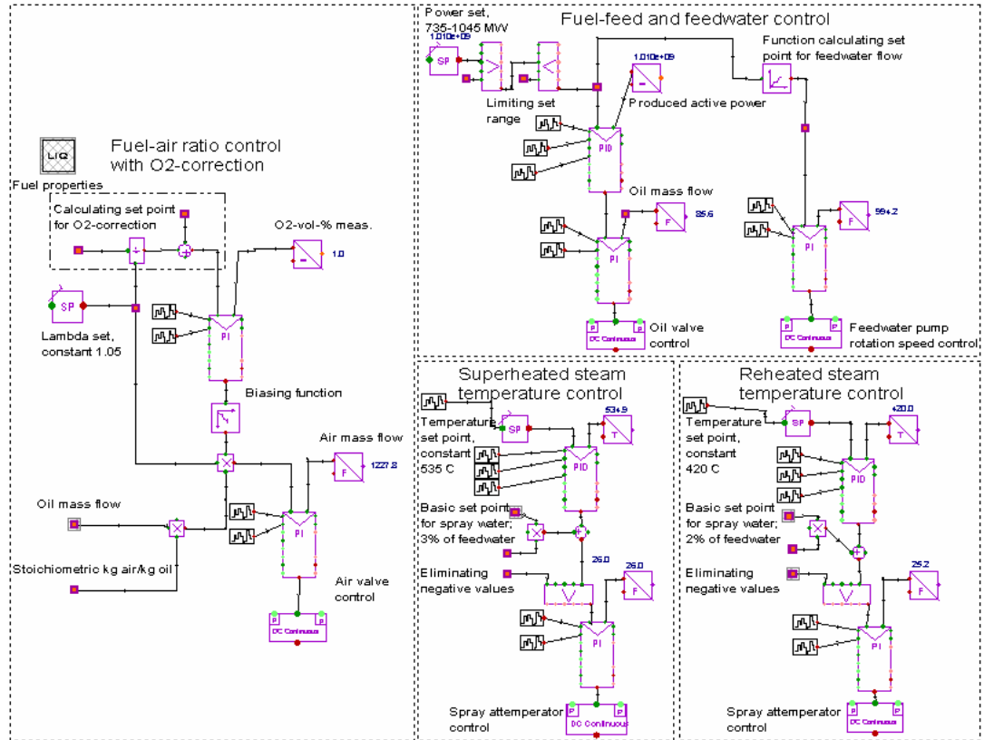
Figure 14. The primary control structures of the power plant model.
