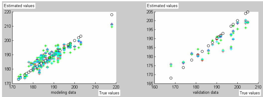
Figure 25. Settling time values from the first iteration step. The PLS estimates are denoted with blue asterisks, PCR with red, CCR with green and CR estimates with cyan. Black circles denote the true obtained values of settling time.
