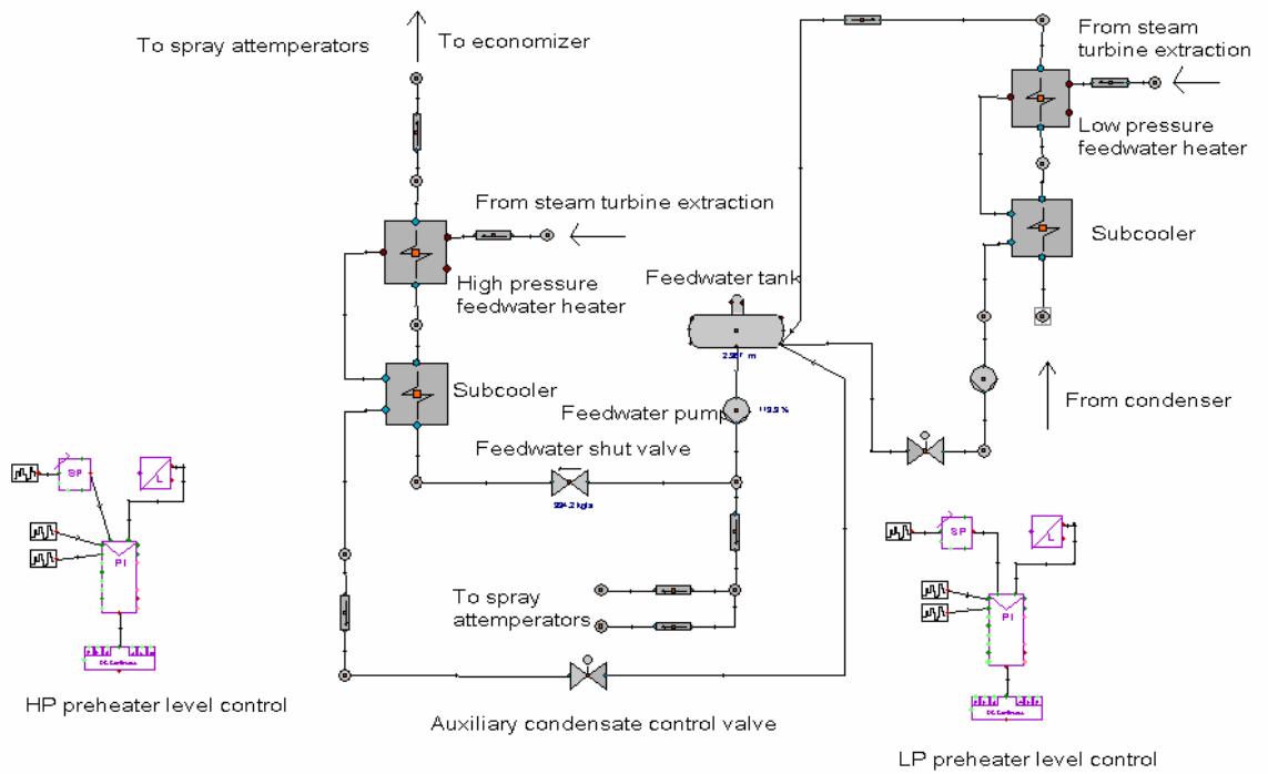
Figure 13. The feedwater section of the power plant model.
