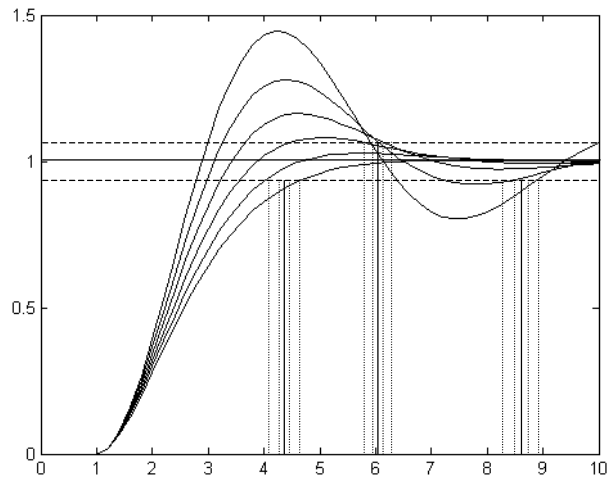
Figure 21. Six step responses of a second order system with different values of damping coefficient. The settling time distribution, if defined through tolerance boundaries, is divided into three separate clusters.
