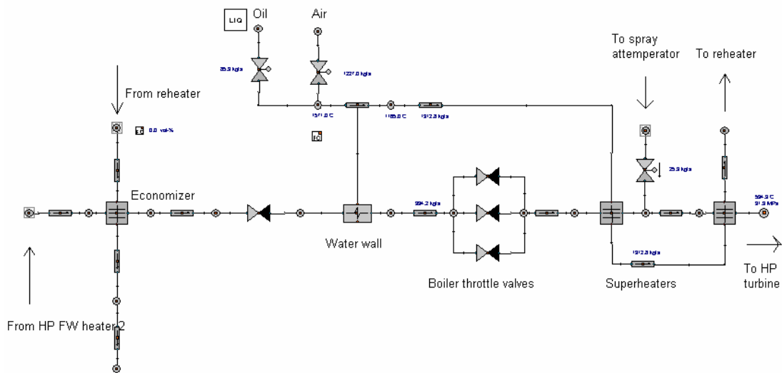
Figure 11. The boiler section of the power plant model.
