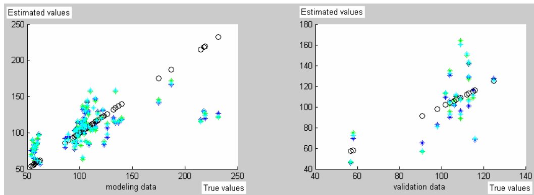
Figure 26. Settling time values from the 20th iteration step. The PLS estimates are denoted with blue asterisks, PCR with red, CCR with green and CR estimates with cyan. Black circles denote the true obtained values of settling time.
