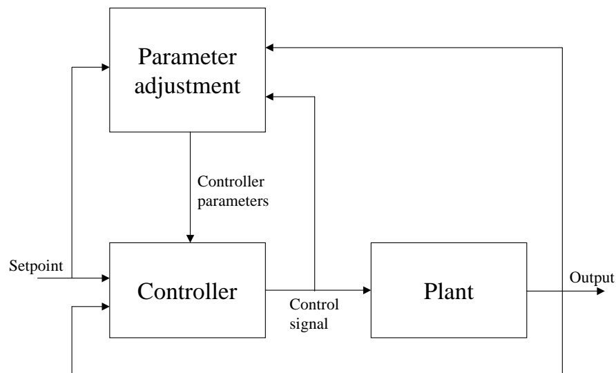
Figure 5. The basic structure of adaptive control /39/.
