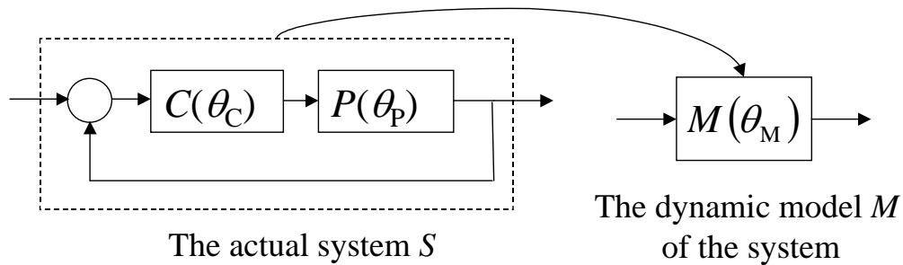
Figure 9. The data obtained from the actual system S can be used for the tuning of the model parameters \theta_M .
