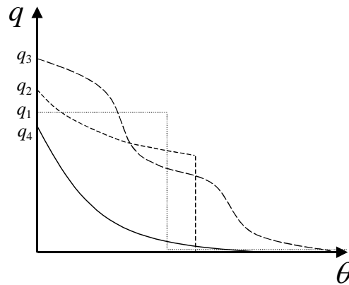
Figure 4. The qualities q_3 and q_4 represent good examples of quality measures whereas one cannot determine the gradient direction of q_1 . Also quality measures of type q_2 are problematic.
