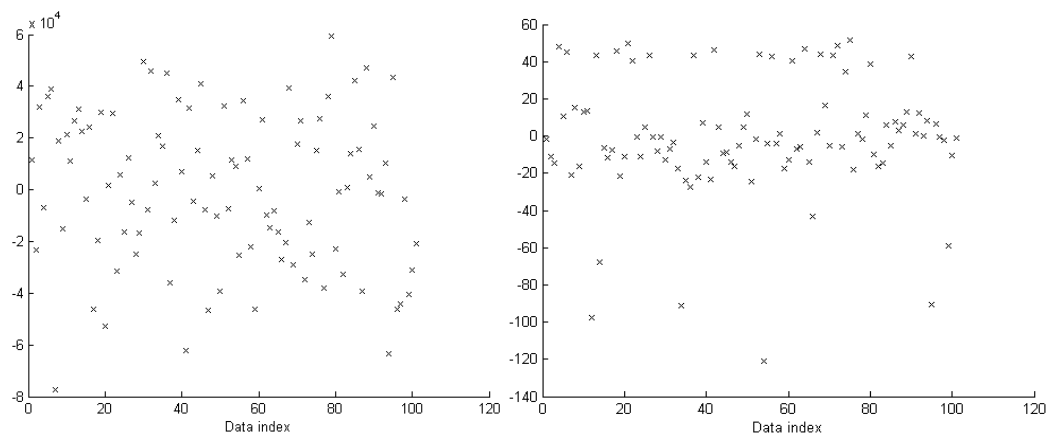
Figure 22. The values of quality measures that are approximately normally distributed (on the left) and divided into three clusters (right).
