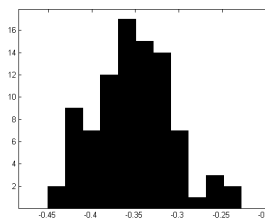
Figure 20. The histogram of the settling time values after the out-of-line data is removed.
