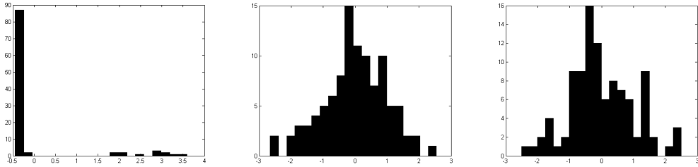
Figure 19. Histograms of the three quality measures, q_1 , q_2 and q_3 , k = 100 .
