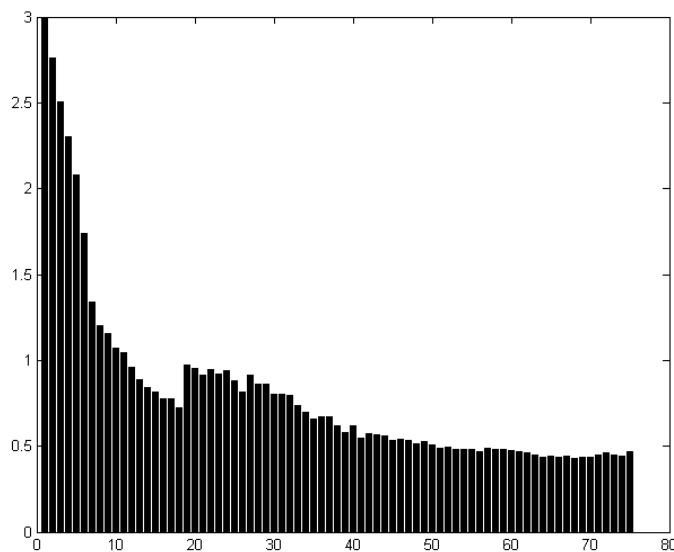
Figure 16. The development of the values of the overall cost function during 75 global iteration steps.
