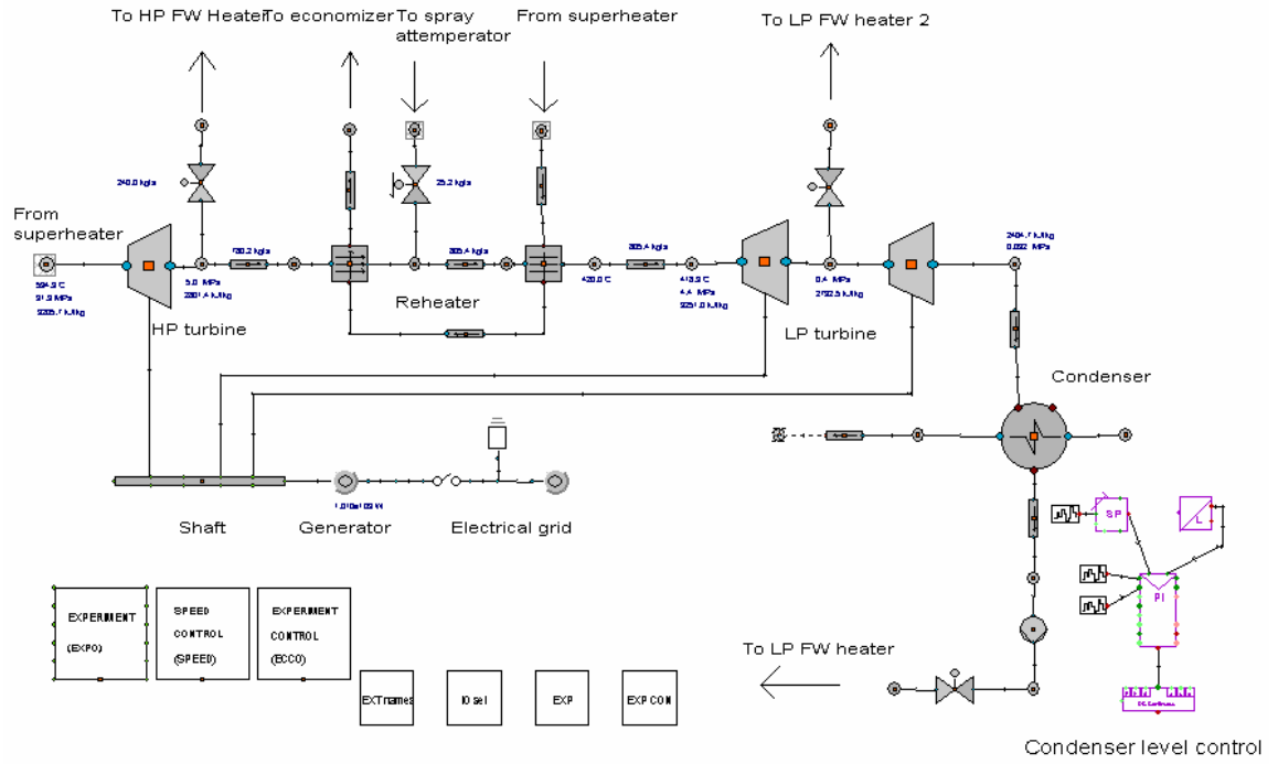
Figure 12. The turbine section of the power plant model.
