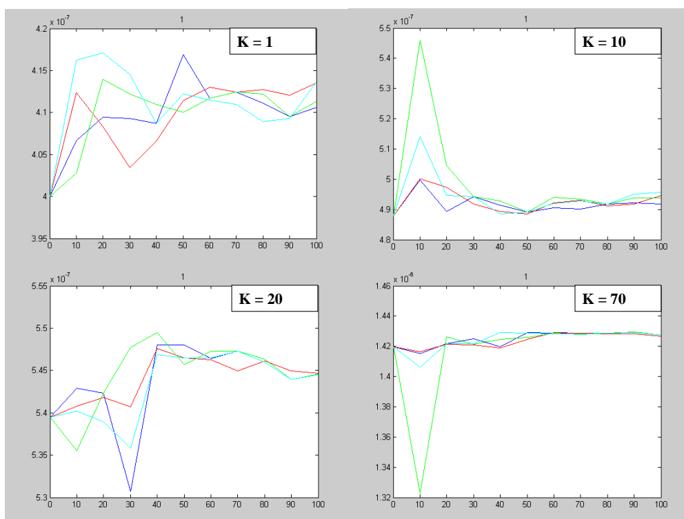
Figure 27. The convergence of the parameter update for \theta_1 on iteration steps K = 1, 10, 20 and 70 subject to the number of the data points. (Red line is the PCR, blue PLS, green CCR and cyan CR proposal.)
