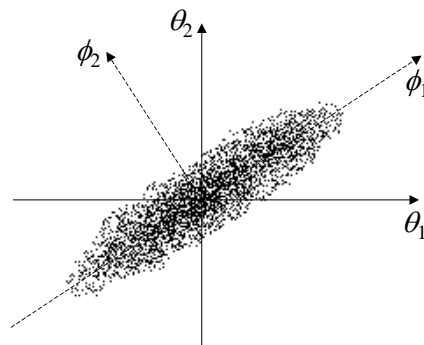
Figure 28. A data distribution in two dimensions: variables \theta_1 and \theta_2 are mutually correlated, i.e., collinear. The same data distribution can be expressed also as a function of \phi_1 and \phi_2 .
