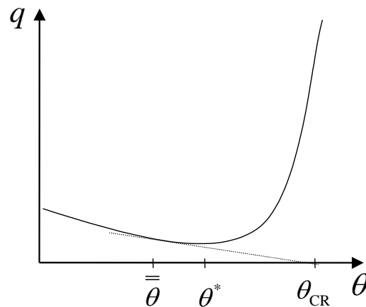
Figure 24. The optimal value of the quality measure q is achieved with the parameter value \theta^* . As \theta^* is passed by and \theta_{CR} is approached the performance starts to degrade fast.
