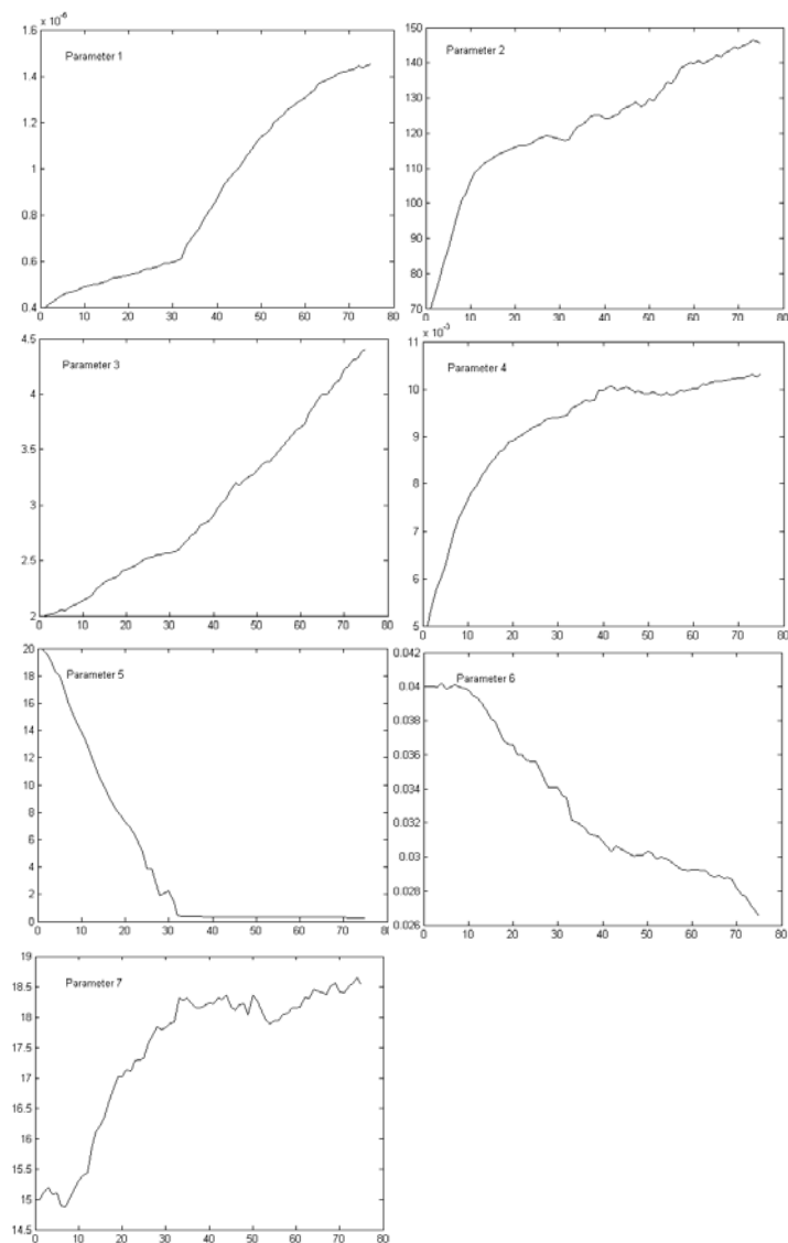
Figure 18. The update trends of the parameters \theta_1 , \theta_2 , ..., \theta_7 during 75 global iteration steps.
