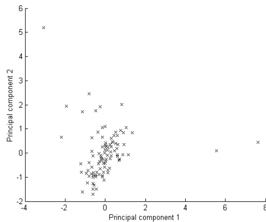
Figure 23. A quality measure distribution from an iteration step involving some out-of-line data points. The data is projected to a plane spanned by its two major principal components.
