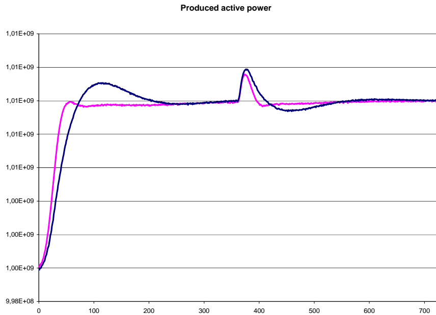
Figure 15. The responses of the produced active power to a setpoint change taking place at the time instant t = 0 s and to a pressure stroke in the combustion ( t = 360 s) before (blue) and after (pink) 18 iterative tuning steps.
