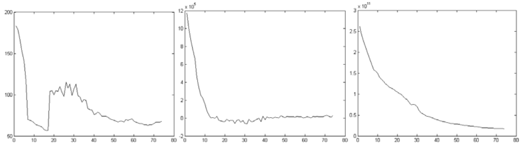
Figure 17. The development of the quality measure values, q_1 , q_2 and q_3 , during 75 global iteration steps.
