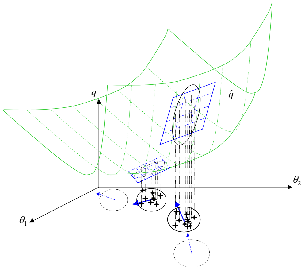
Figure 6. The optimization procedure consists of K successive global iteration steps (in this figure, K = 4 ). During each step, k data points are produced in local iteration. The data is used for modeling the local interdependence between the parameters \theta and the quality measures q .
